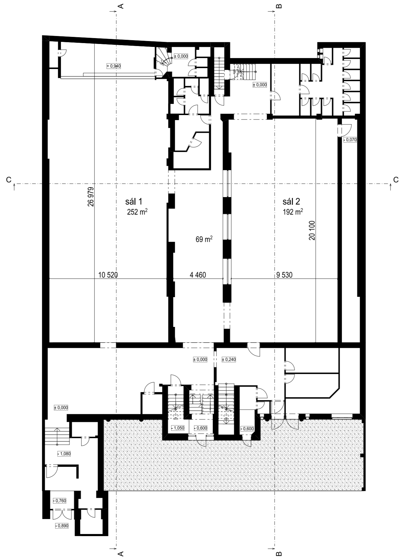
pūdorys, 1. patro / floorplan of the ground floor – 1:200
