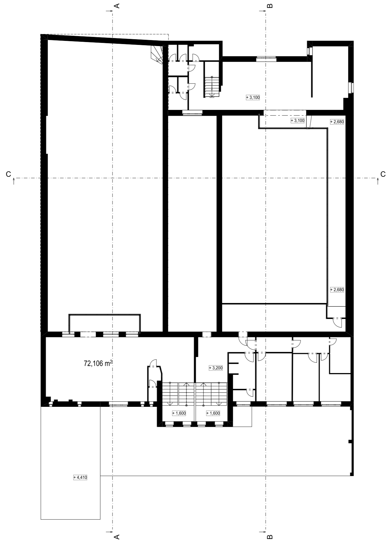
pūdorys, 2. patro / floorplan of the first floor – 1:200
